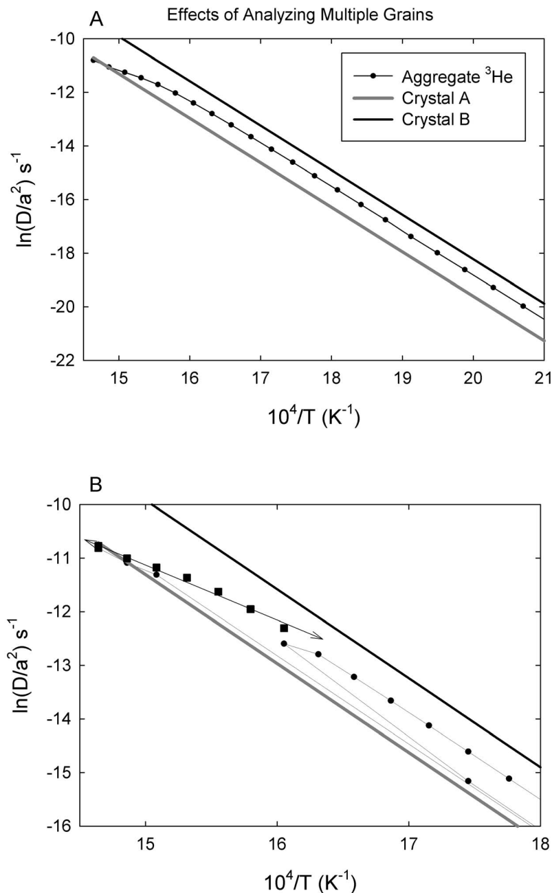
Figure 7. Arrhenius plots simulated for a two-crystal aggregate with D_A/D_B = 4 and a uniform and identical concentration of helium in the two crystals. (a) Comparison of the results obtained on the aggregate to the diffusivities assumed for the individual grains, assuming a monotonic heating schedule spanning a large temperature range. The aggregate diffusivity is curved because it is initially dominated by the less retentive grain, but as the experiment proceeds this grain becomes depleted and the diffusivity declines toward that of the more retentive grain. (b) Comparison starting with the same assumptions as in Figure 7a but using two different heating schedules described in section 3.5. These simulations show that mixtures of grains with different diffusivities analyzed together need not yield accurate diffusion parameters (as suggested by arrow in Figure 7b). The telltale signs of this effect are a curved Arrhenius array and, for cycled experiments, a declining zigzag pattern.
