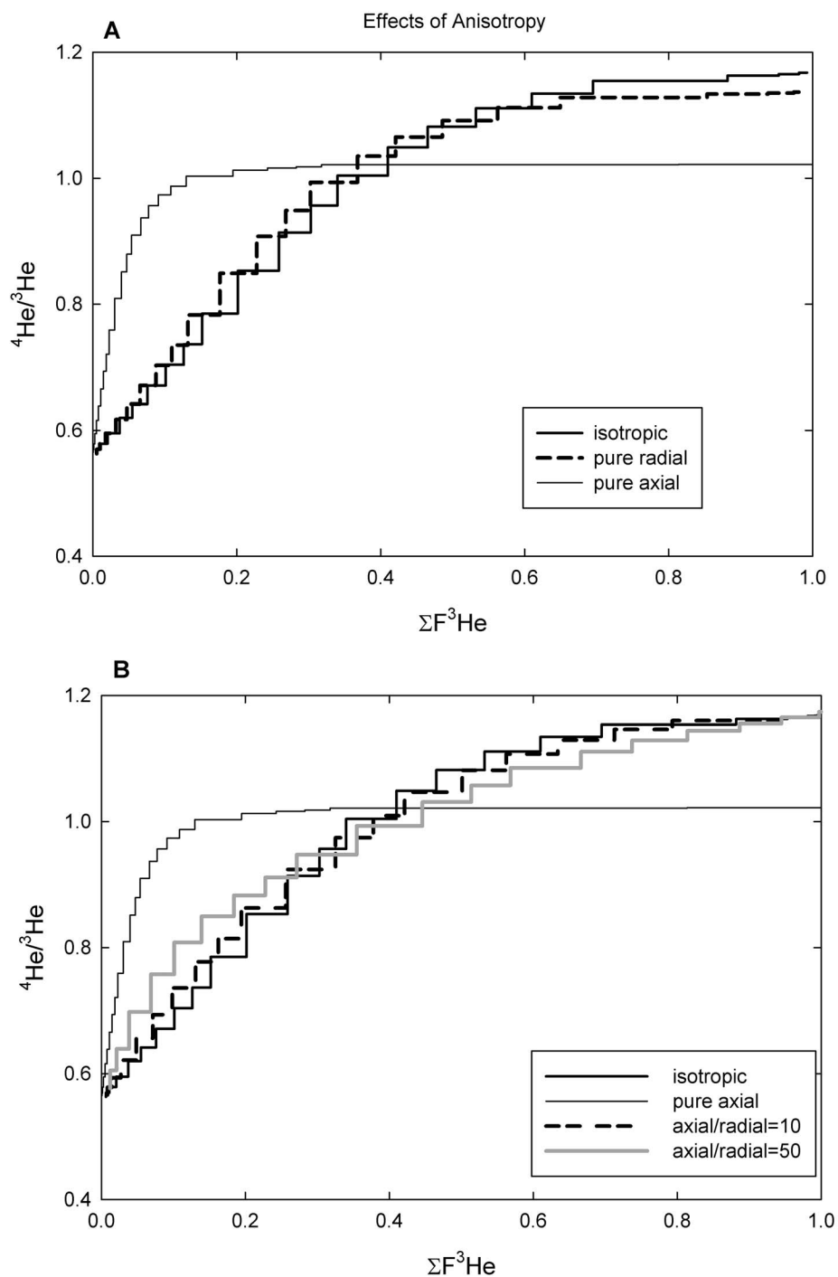
Figure 3. Comparison of ^4\text{He}/^3\text{He} spectra obtained from a 330 \times 55 \mu\text{m} cylinder assuming varying degrees of anisotropic diffusion from an \alpha ejection-only starting condition. (a) Results for isotropic diffusion, pure axial diffusion, and pure radial diffusion. While pure axial diffusion yields a very different ^4\text{He}/^3\text{He} spectrum compared to the isotropic case, pure radial diffusion is almost indistinguishable from the isotropic case. (b) Demonstration that ^4\text{He}/^3\text{He} spectra become noticeably different from the isotropic case when the ratio of axial to radial diffusion exceeds about 10. Although data are limited, there is no evidence for this magnitude of anisotropy in apatite.
