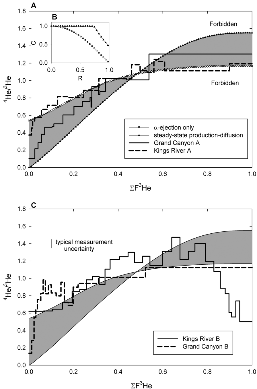
Figure 1. Limiting ^4\text{He}/^3\text{He} spectra and examples. (a) Spectra for the two limiting cases of \alpha ejection-only and production-diffusion- \alpha ejection steady state evolved from (b) the limiting concentration profiles ( C , normalized concentration; R , normalized radial coordinate). All ^4\text{He}/^3\text{He} spectra that conform to assumptions (see section 1 for details) must lie within uncertainty of the shaded region and not in the regions labeled “forbidden.” Also shown in Figure 1a are two spectra that plot within error of the allowed region. (c) Two obviously anomalous measured ^4\text{He}/^3\text{He} spectra (sample and data details in Data Set S1). These spectra were measured on multiple grain aliquots. Note that measured spectra are plotted as a series of steps reflecting the amount of gas released in each step, whereas the model curves here are continuous curves that would apply to very small steps. For clarity the uncertainties on measured data are not shown, but a typical 1\sigma uncertainty estimate is indicated in Figure 1c.
