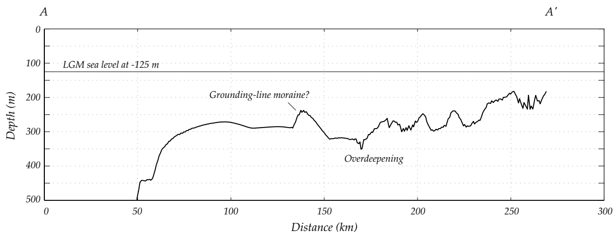
Figure 3. Bathymetric profile down the axis of the prominent elongated trough, crossing the suggested grounding line moraine complex. The location is shown on Figure 2. The data in the overdeepened region are noisy due to crossings of fathometer lines from varying data sources that appear to have been inconsistently processed; this can be seen by comparing Figures 2 and 3.
