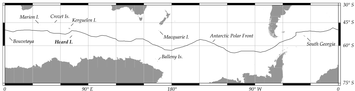
Figure 1. The islands of the Southern Ocean. The mean location of the Antarctic Polar Front is from Moore et al. (1999).
